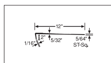
Service Weight Square Nose (ST)
