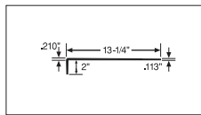
Rice Paper Tread (FRPT)
