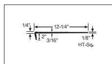
Safe-T-Rib® Square Nose (HT)
