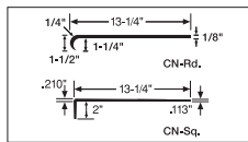
Heavy Duty Diamond Tread (CN)
