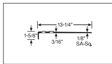
Service Weight Safe-T-Grip Tread (SA)
