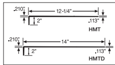
Hammered Tread (HMT) 12 1/4" deep (HMTD) 14" deep
