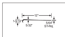
Service Weight Round Nose (ST)
